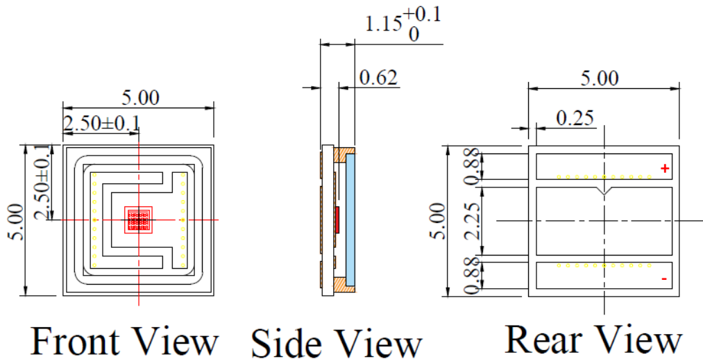
VD-0940I-002W-1D-2A0 (substrate AlN, 5050 packaging), unit:mm
