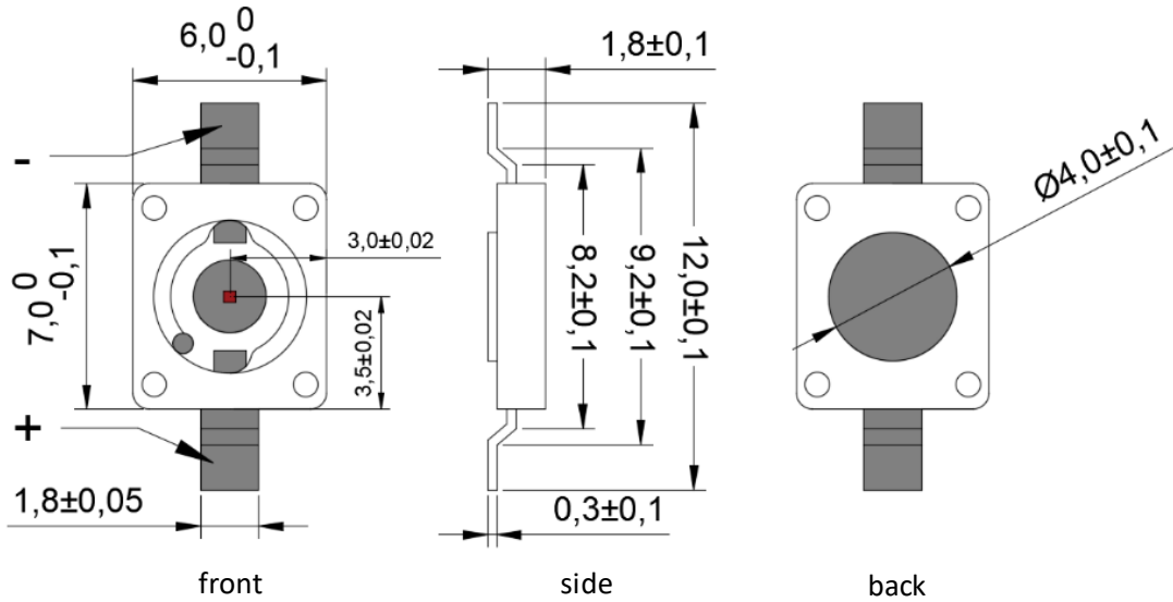
VD-0940I-002W-1E-2A0 (substrate AlN, 7060 packaging), unit:mm
