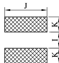
( PCB Pattern )
