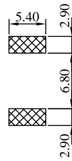
(PCB Pattern)
