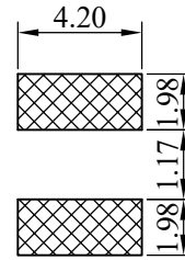
( PCB Pattern )
