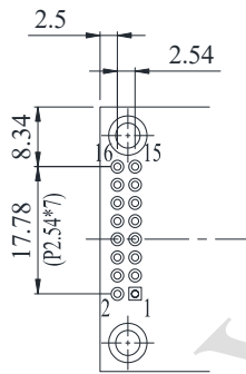
PIN DETAIL
