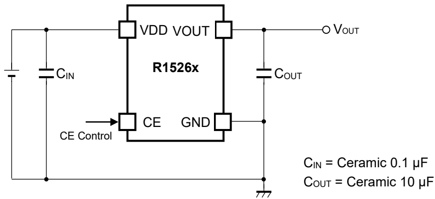
Test Circuit for Typical Characteristics
