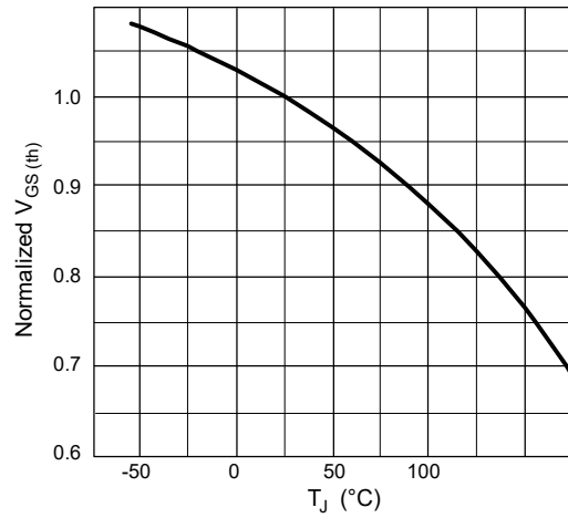
FIG. 2-Normalized V_{GS(th)} vs T_J
