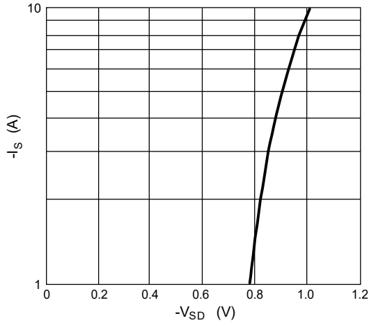
FIG. 1-Forward Characteristics of Body Diode
