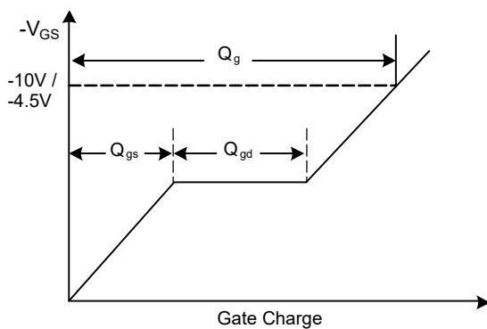
FIG. 5-Gate Charge Waveform
