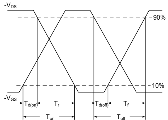
FIG. 4-Switching Time Waveform
