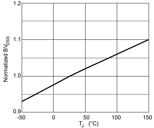
FIG. 2- Normalized BV DSS vs. T J
