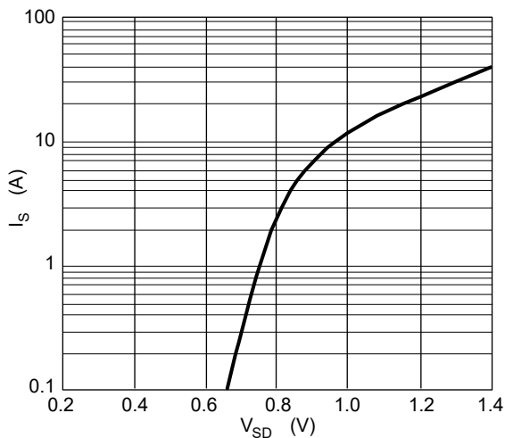
FIG. 5- Drain-Source Diode Forward
