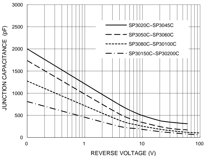
FIG. 5-TYPICAL JUNCTION CAPACITANCE
