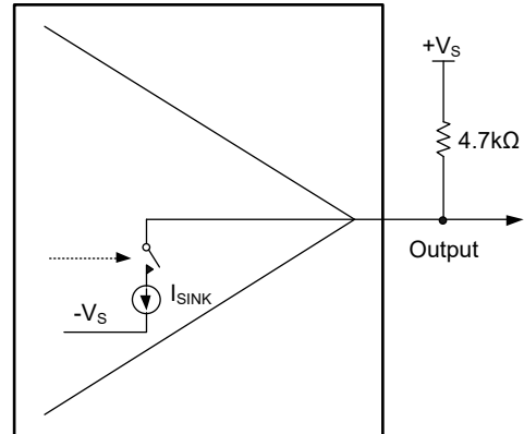
Figure 1. SGM8778A/B/C/D-1 Open-Drain Output Structure
