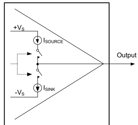
Figure 2. SGM8778E-1 Push-Pull Output Structure
