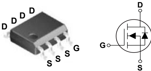
SOP-8 Pin Configuration
