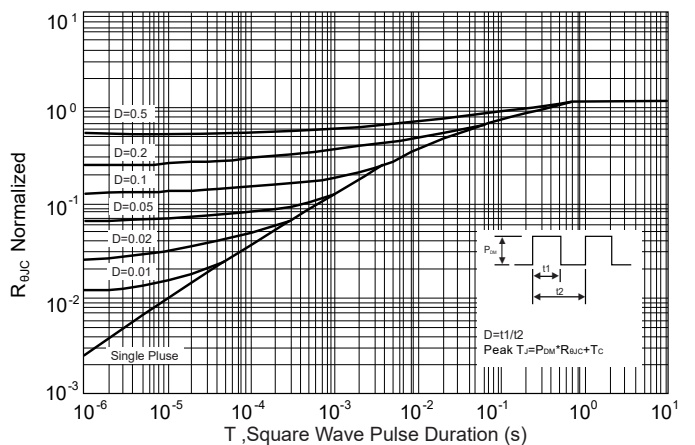
FIG. 6 - Normalized Transient Impedance
