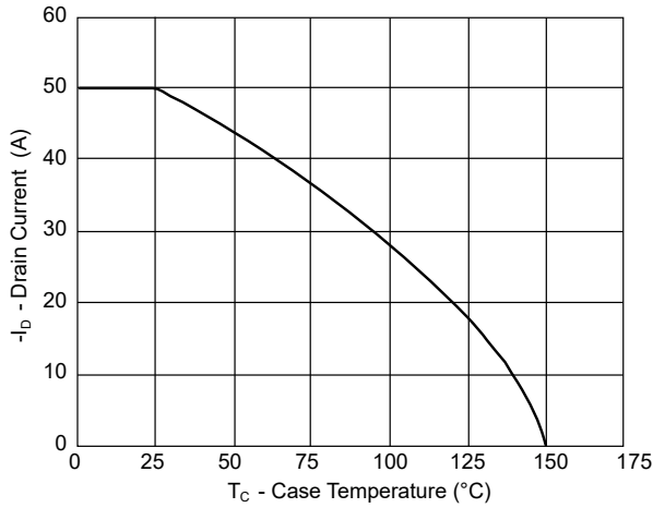
FIG. 1 - Drain Current vs. T_C
