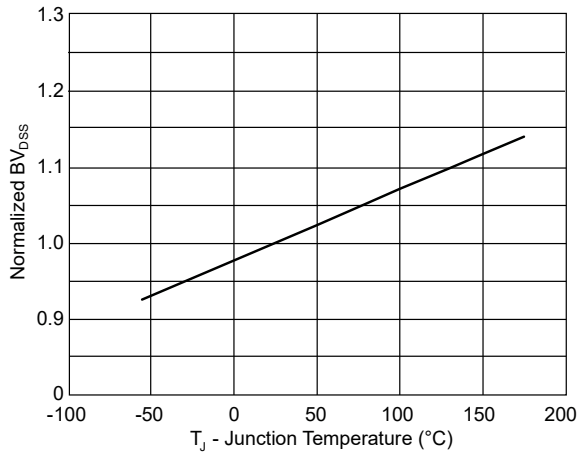
FIG. 3 - Normalized BV DSS vs. T J
