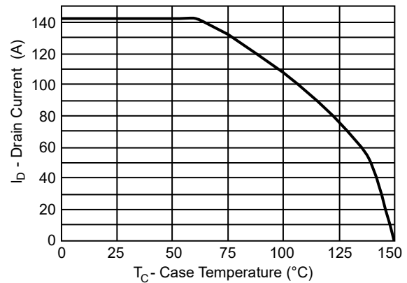
FIG. 4- Drain Current
