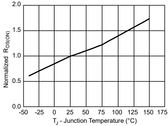
FIG. 1- Drain-Source On-Resistance
