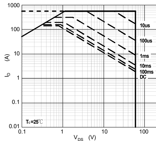
FIG. 6- Safe Operation Area
