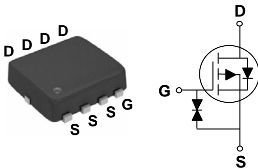
PPAK3X3 Pin Configuration
