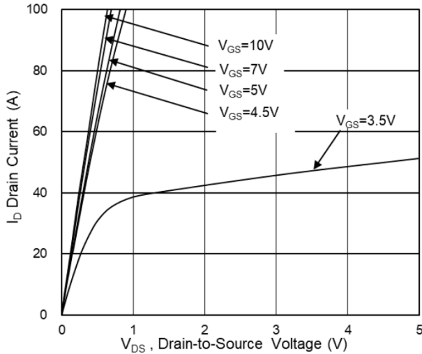
FIG.1-Typical Output Characteristics
