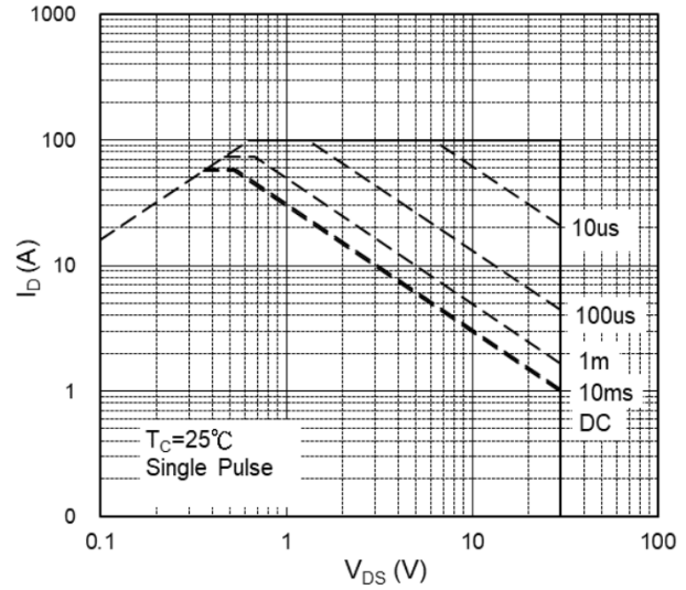
FIG.8-Safe Operating Area
