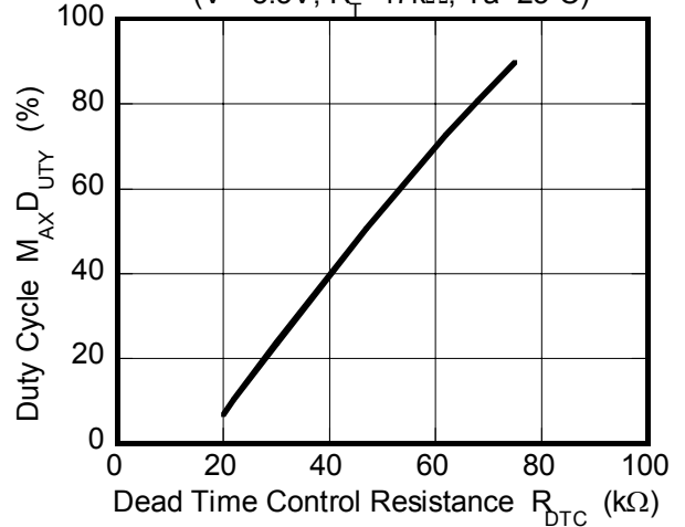
Duty Cycle vs. R_{DTC}
