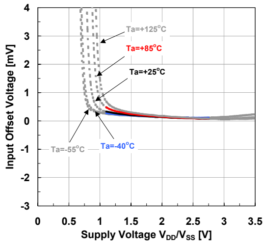
Input Offset Voltage vs. Supply Voltage (Ambient Temperature) No Signal, A_v=0dB
