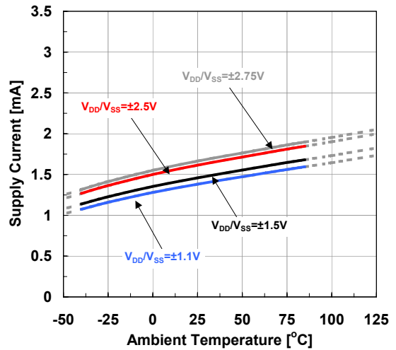
Supply Current vs. Ambient Temperature No Signal, A_v=0dB
