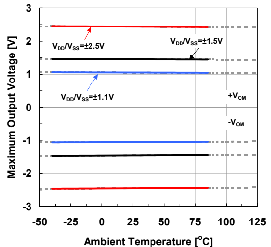
Maximum Output Voltage vs. Ambient Temperature G_v = OPEN , R_L = 600\Omega
