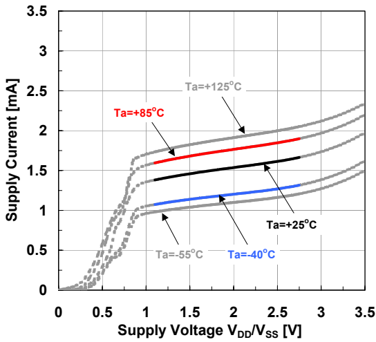
Supply Current vs. Supply Voltage (Ambient Temperature) No Signal, A_v=0dB
