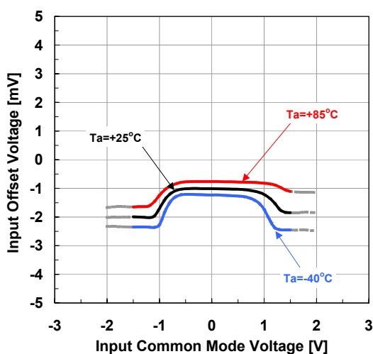
Input Offset Voltage vs. Input Common Mode Voltage V_{DD}/V_{SS} = \pm 1.5V , R_L = 10k\Omega
