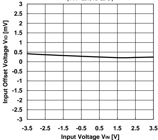
Input Common Mode Voltage Range (V+/V-=±5V, Ta=25°C)
