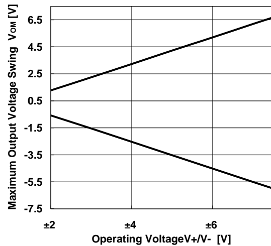
Maximum Output Voltage Swing vs. Operating Voltage (Ta=25°C)
