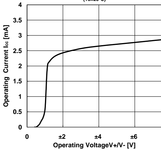
Operating Current vs. Operating Voltage (Ta=25°C)
