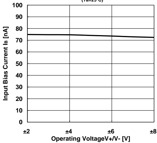
Input Bias Current vs. Operating Voltage (Ta=25°C)
