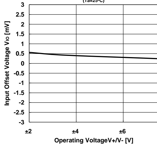
Input Offset Voltage vs. Operating Voltage (Ta=25°C)
