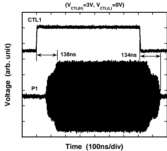
Switching Time Characteristic
