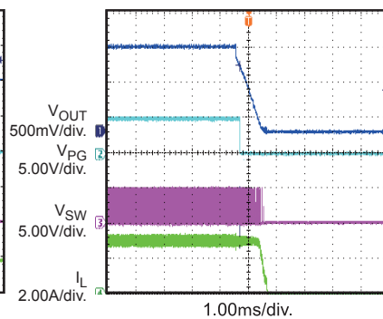
Power Good Off with 3A Load
