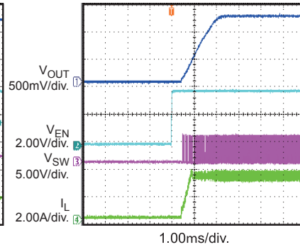
EN Start Up with 3A Load
