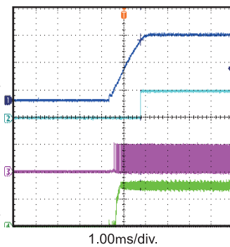
Power Good On with 3A Load
