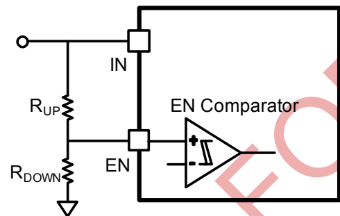
Figure 9: Adjustable UVLO
