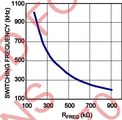
Switching Frequency vs. R FRQE
