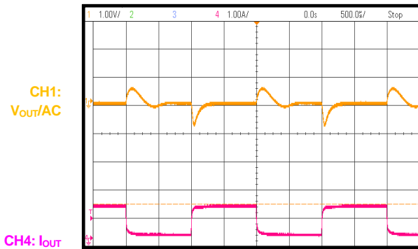
Load Transient I_{OUT} = 0A to 1A , I_{RAMP} = 25mA/\mu s
