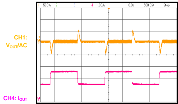
Load Transient I_{OUT} = 1A to 2A , I_{RAMP} = 25mA/\mu s
