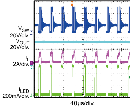
Mixed Dimming via the I 2 C Interface D DIM = 20%
