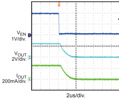
EN Shut Down with Resistive Load I_{OUT}=250mA
