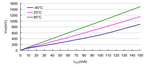
Dropout voltage: HT7550-7
