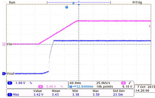
Power On Response: HT7533-7 ( I_{OUT}=100mA , T_{RISE}=100ms )
