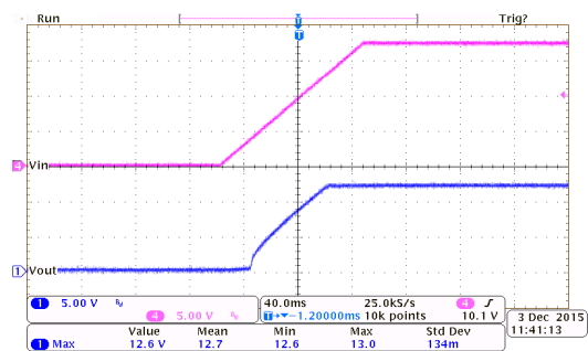
Power On Response: HT75C0-7 ( I_{OUT}=150mA , T_{RISE}=100ms )
