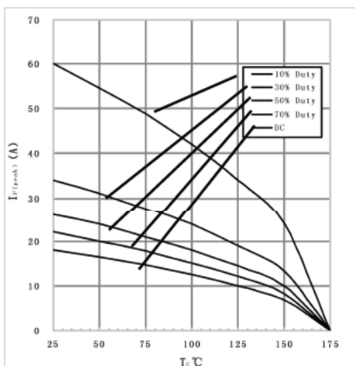
3) Current Derating
