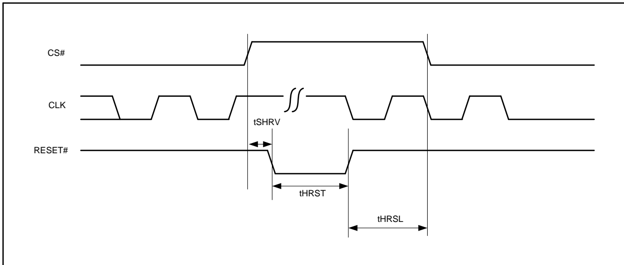
Figure 46. Reset Timing
