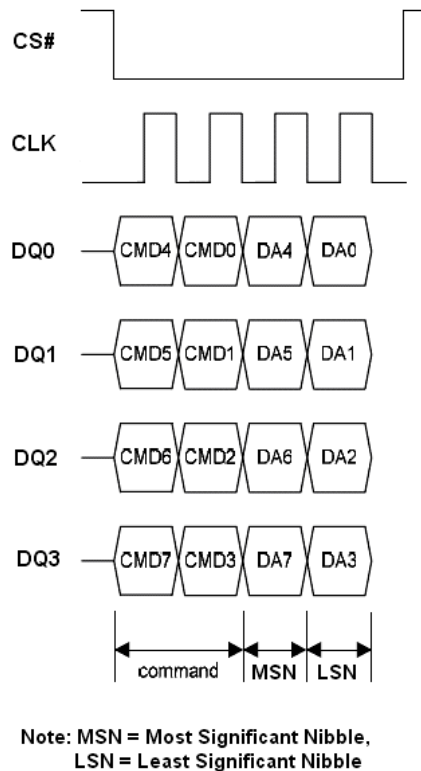
Figure 23.1 Write Status Register 2 Instruction Sequence Diagram in QPI mode
