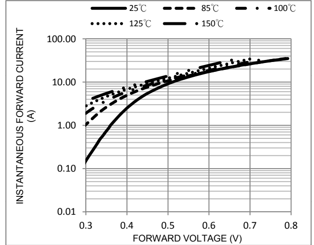
FIG. 2-Typical Forward Characteristics
