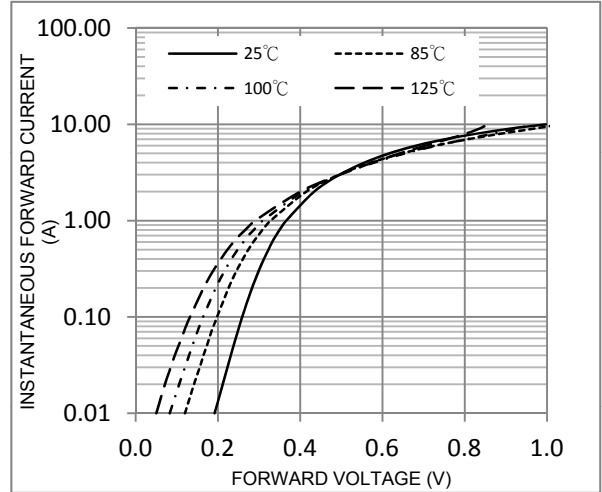
FIG. 2-Typical Forward Characteristics
