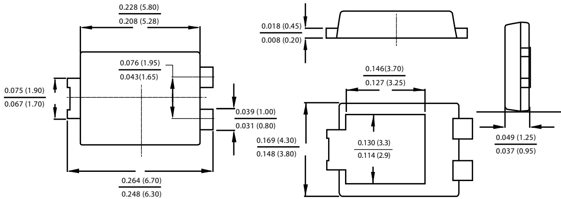
TO-277
