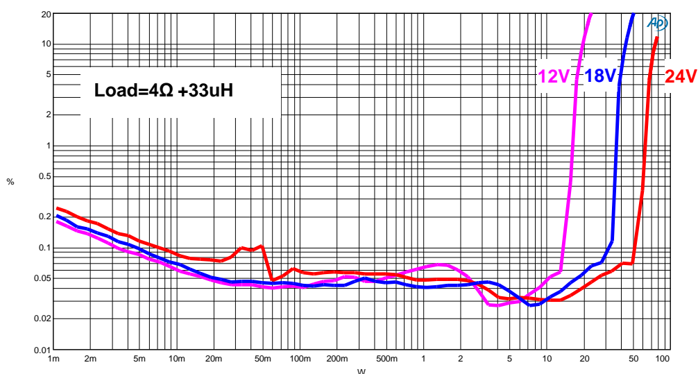
THD + N (%) v.s. Output power (Mono 4Ω load)
